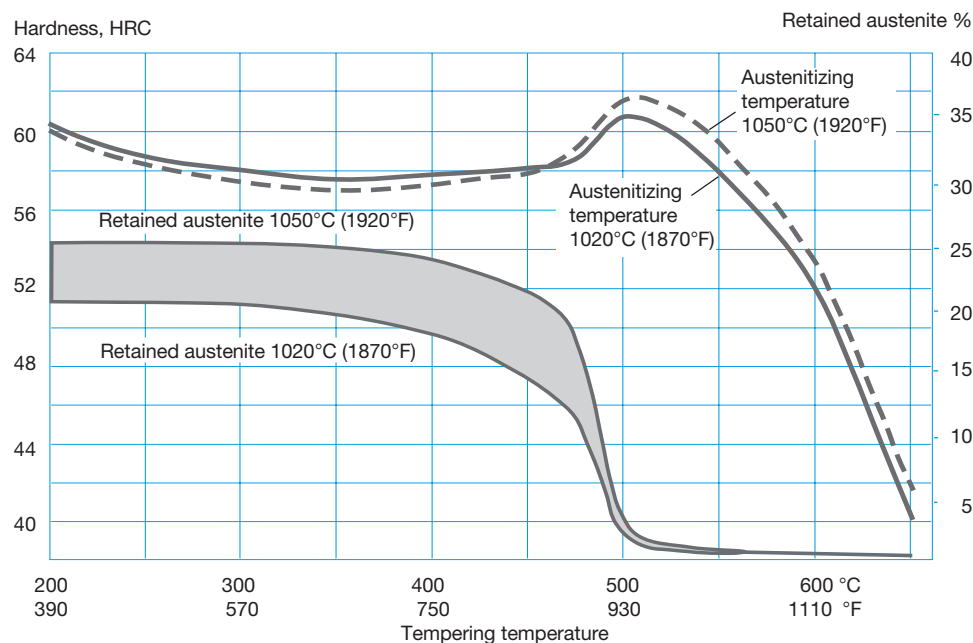
TEMPERING GRAPH
